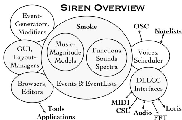
Figure 1. Siren Framework Overview
