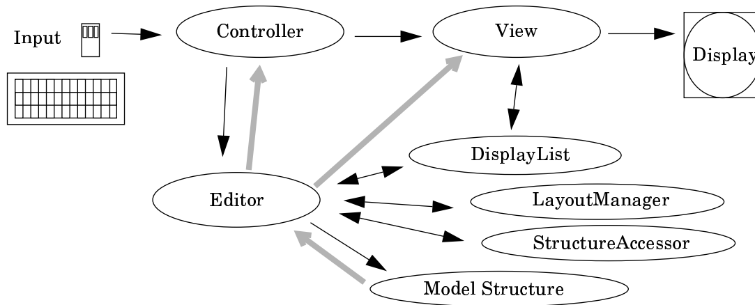
Figure 6: Navigator MVC Software Architecture
