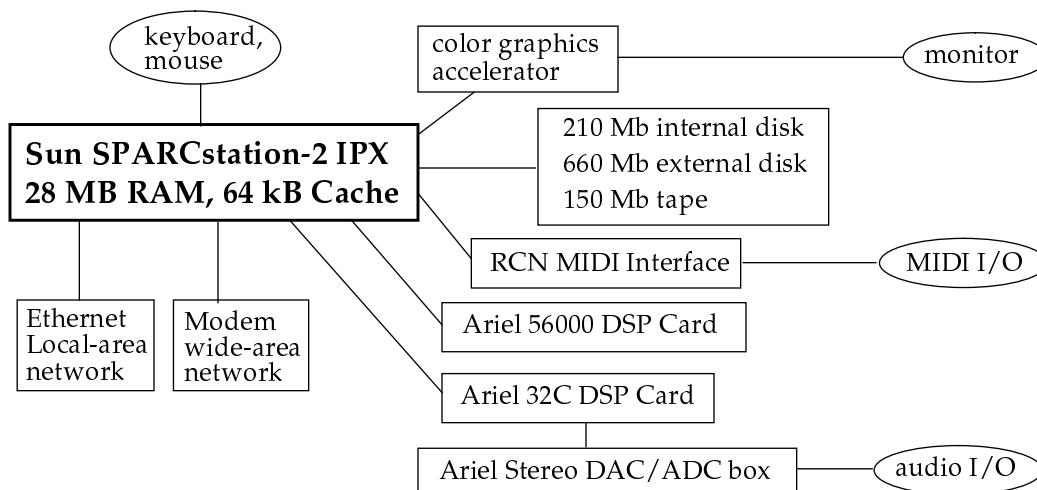
Figure 1: Current IDP hardware configuration
